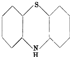
Thiodiphenylamin.
